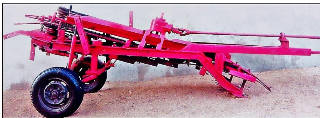
Fig. 4. Developed harvesting machine for onion crop (Nour et al., 2020)
