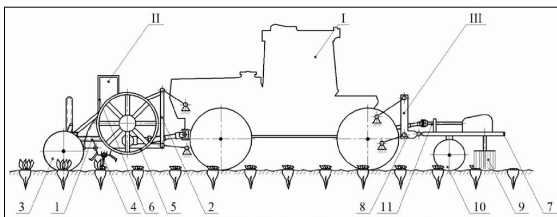
Fig. 2. Schematic diagram of beet tops harvesting machine (Ye, 2017)
