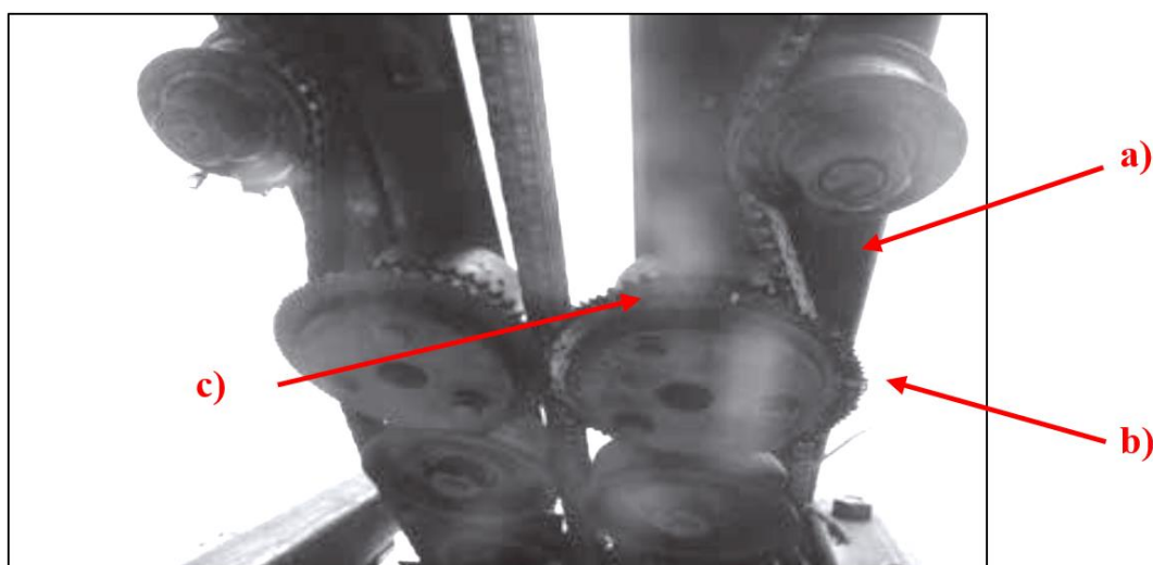
Fig. 3. De-topping unit of the developed carrot digger (Rani et al., 2018)
