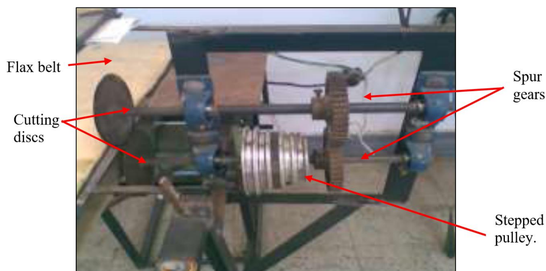
Fig. 6. Trimming unit of green onion crop handling mechanism (Mayhoub et al., 2009)
